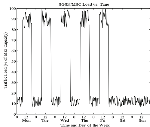
Fig. 2. Representative SGSN/MSC Load
