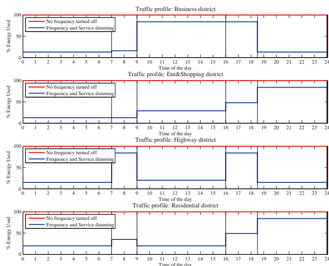
Fig. 6. Percentage of Maximum Power Consumption Vs. Time for Various Types of Cells with Frequency and Service Dimming
